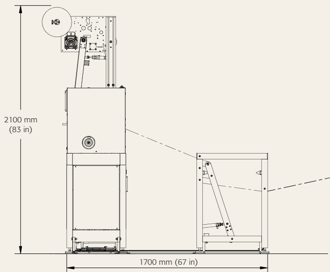
HSW 550/32
